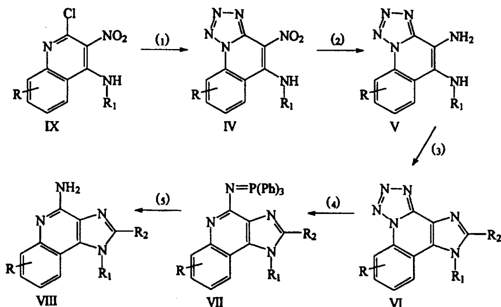
Reaction Scheme II
